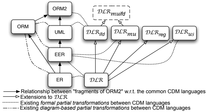
Fig. 2. Relations between common conceptual data modeling languages and the DLR family of Description Logic languages; \mathcal{CM}_{com} has an equi-satisfiable DLR_{ifd} knowledge base. The higher up in the figure, the more constructors available in the language.
